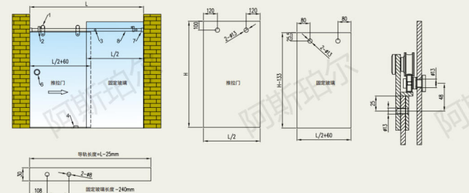
30×10 方管 Illustration for 30×10 Square pipe
