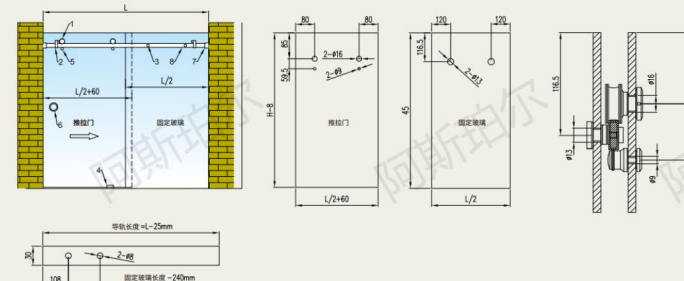
30×10 方管+防跳器 30×10 Square pipe with jumping-proof device
